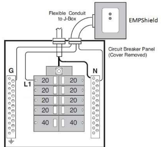
Figure 6 – 240V European Model Wiring
