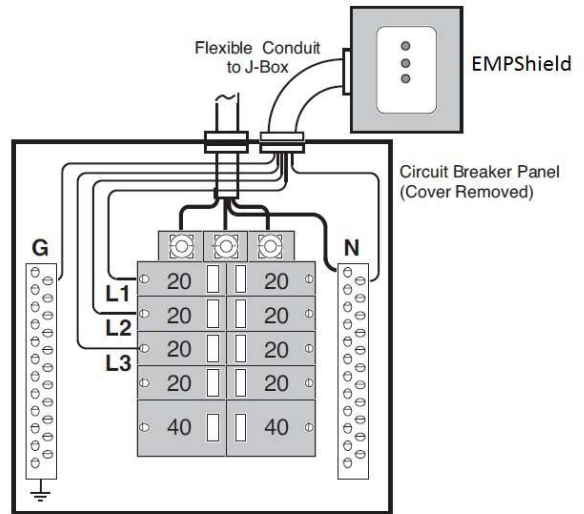
Figure 6 – 240V European Model Wiring
